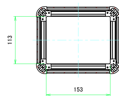
C-C (1:4)
